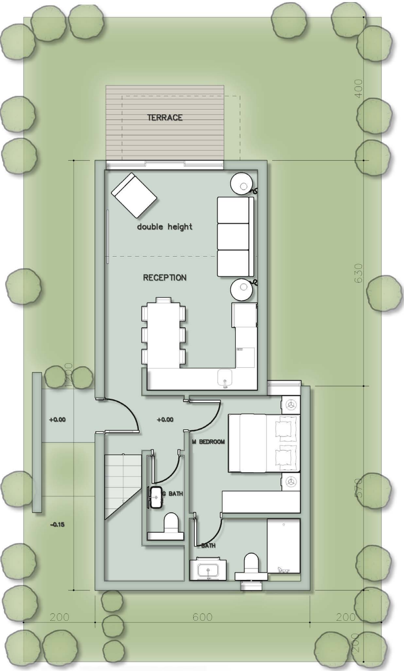
Ground Floor
