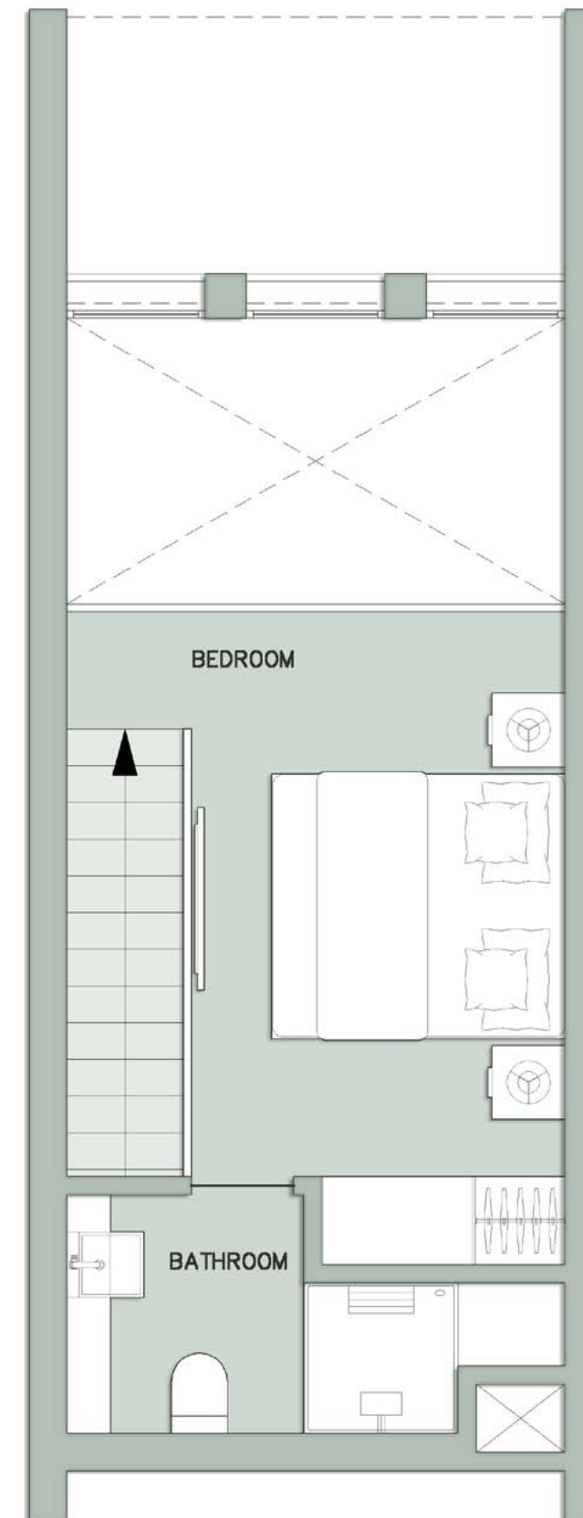
FIRST FLOOR
