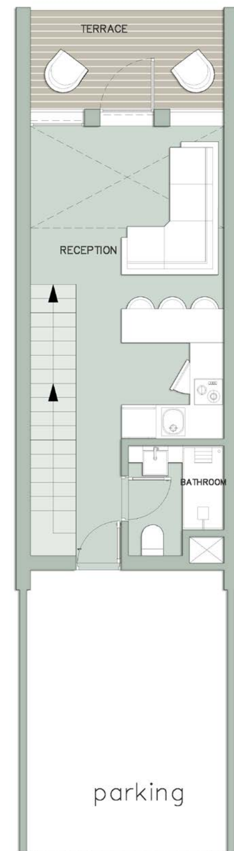
GROUND FLOOR
