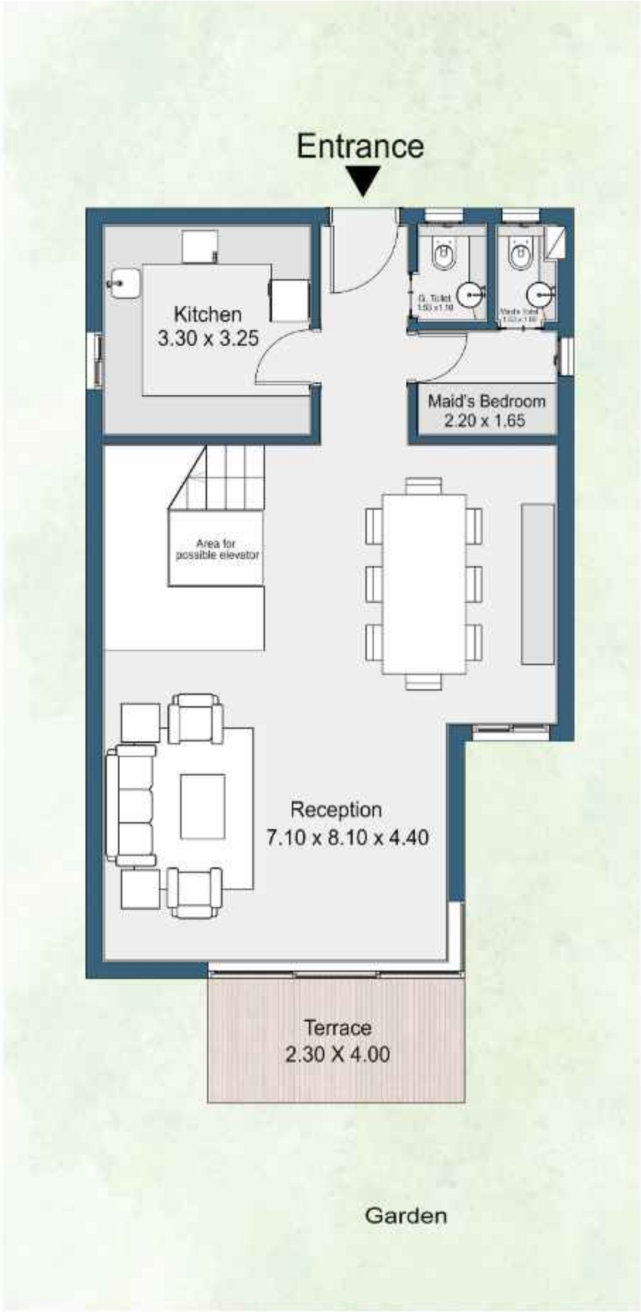
GROUND FLOOR
