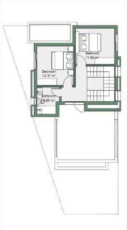
SECOND FLOOR
